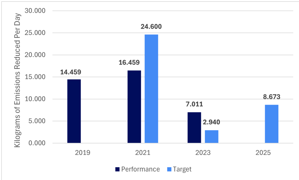
Figure 17 - 2019-2025 CMAQ Emissions Reduction Performance for VOCs
