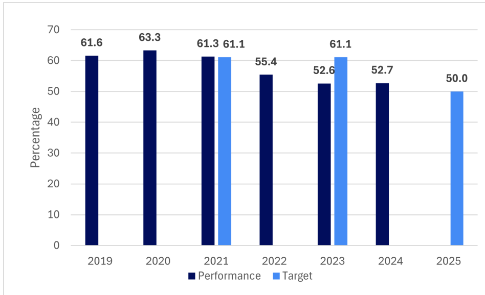
Figure 8 - NHS (Non-Interstate) Pavement: Performance vs. Targets (Good)
